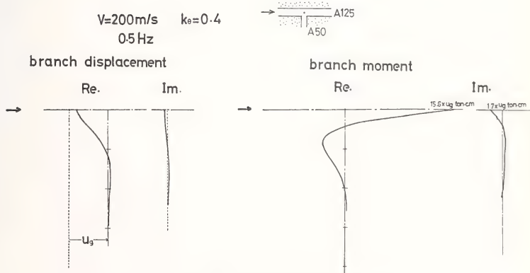
Fig. 10 Displacement and Strain of a Branch Pipe
